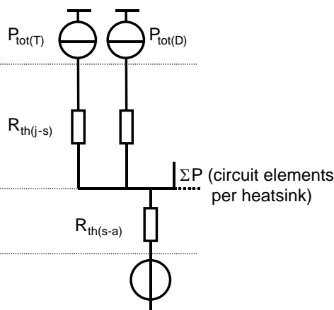
Figure 3.3.10 (Static) thermal models for modules with and without base plate
