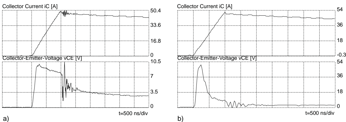
Figure 5.9.9 a) di/dt -impression in a 1200 V / 50 A-NPT-IGBT ( di/dt = 50 \text{ A}/\mu s ; i_L = 50 \text{ A} ) b) di/dt -impression in a 1200 V / 50 A-PT-IGBT ( di/dt = 50 \text{ A}/\mu s ; i_L = 50 \text{ A} )
