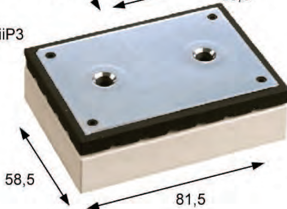
Figure 2.5.47 Standard MiniSKiiP designs (dimensions in mm) and circuits
