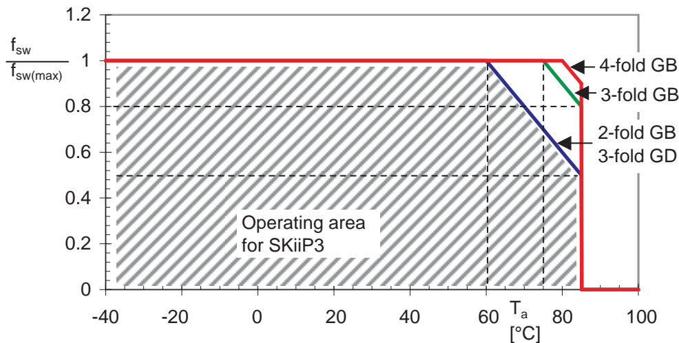
Figure 3.6.7 Derating of the maximum permissible switching frequency of a SKiiP3 at T_a > 25^\circ\text{C}
