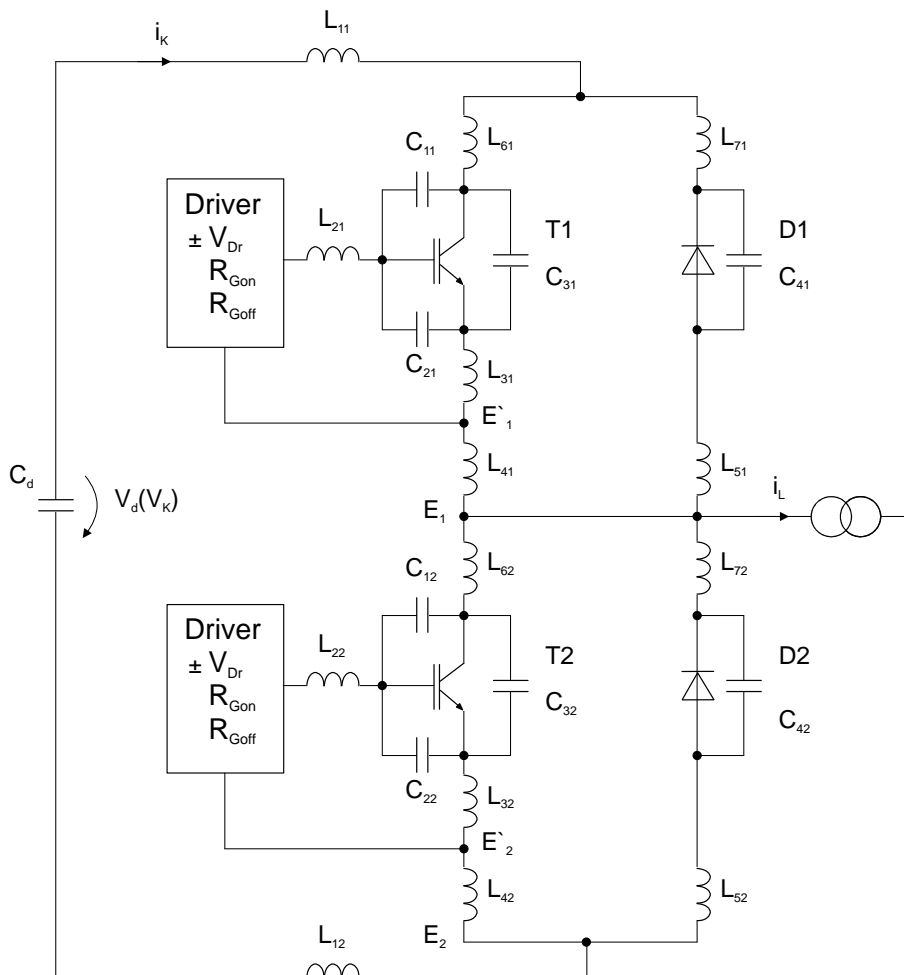
Figure 5.4.1 Commutation circuit with parasitic inductive and capacitive elements
