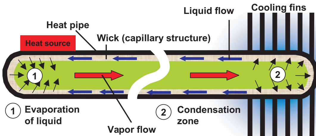
Figure 5.3.24 Principle behind a heatpipe. Since gas and liquid are almost in a balance in (1) and (2) and the same pressure is present, the temperatures in (1) and (2) are almost identical.
