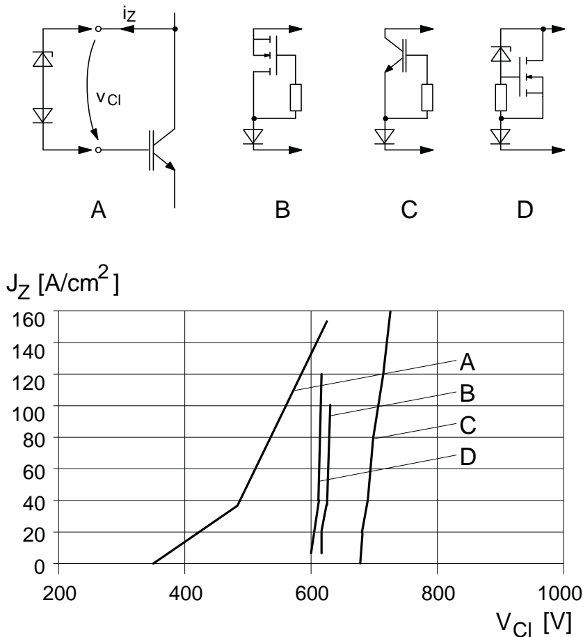
Figure 5.7.17 Static characteristics of selected Zener elements
