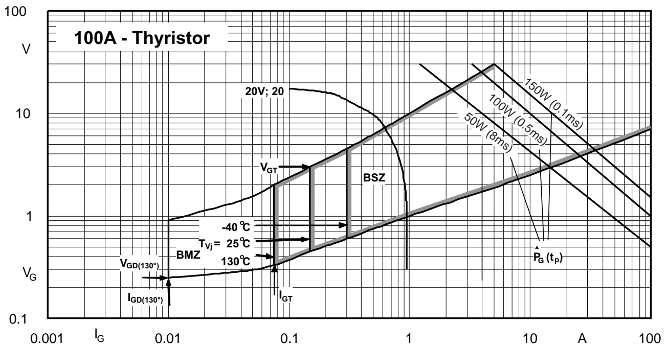
Figure 3.2.21 Trigger current ( I_G ) over trigger voltage ( V_G ) of a 100 A thyristor (spread) with areas of possible and safe triggering. P_G(t_p) is the maximum permissible peak gate power dissipation at a gate current pulse duration t_p ; the curve labelled "20 V; 20 \Omega " is the characteristic of a trigger device for 20 V no-load voltage and 20 \Omega internal resistance.
