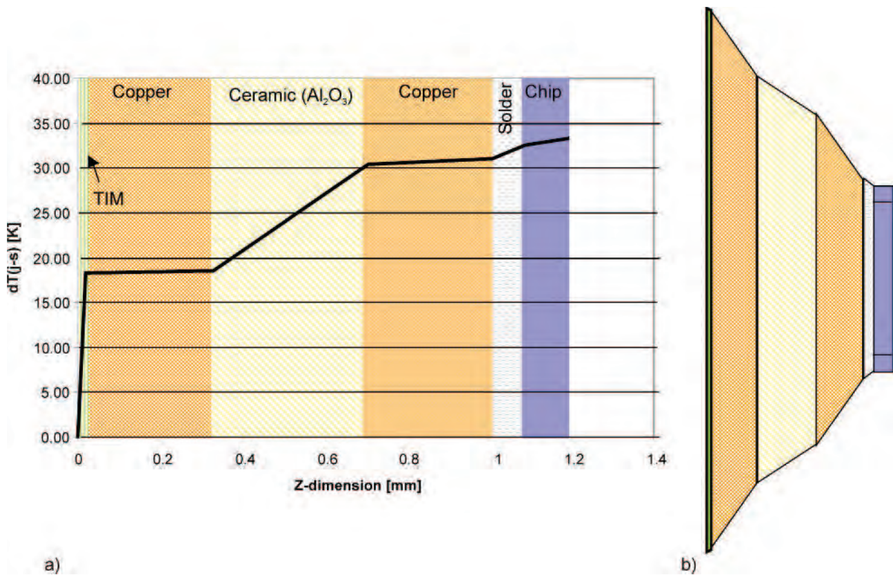
Figure 2.5.15 Layer structure with heat spreading (b) and typical temperature profile (a) for a module without base plate (0.38 mm \text{Al}_2\text{O}_3 ceramic, 25 \mu\text{m} thermal paste, TIM)
