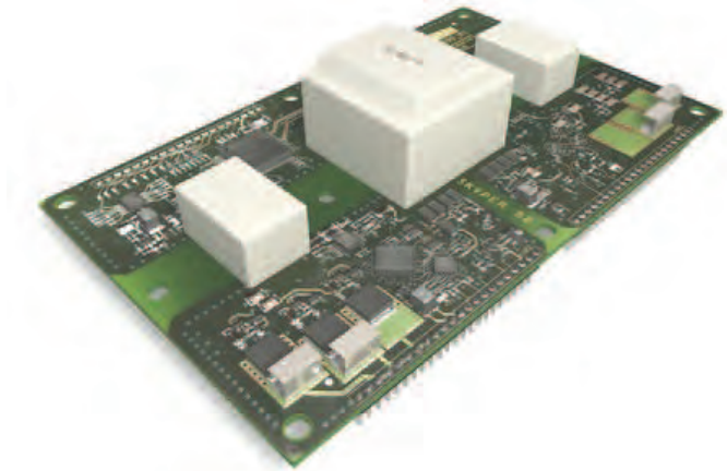
Figure 5.6.16 SKYPER 52 R driver stage PCB
