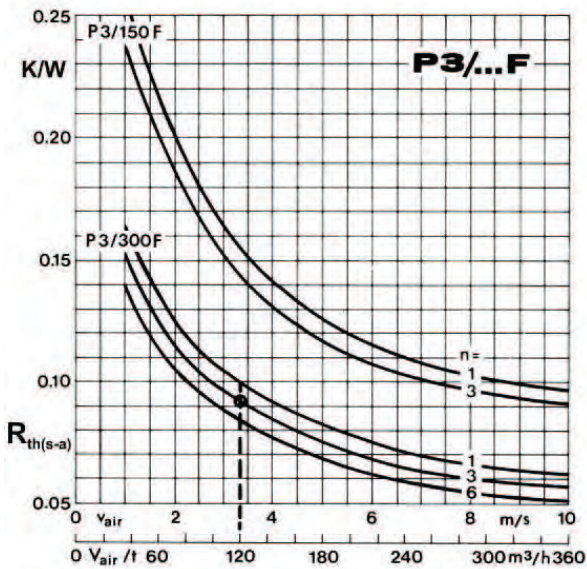
Figure 4.2.11 R_{th(s-a)} for P3 heat sink profile in different lengths, equipped with n = 1 - 6 components, as a function of the air volume V_{air}/t or air velocity v_{air}
