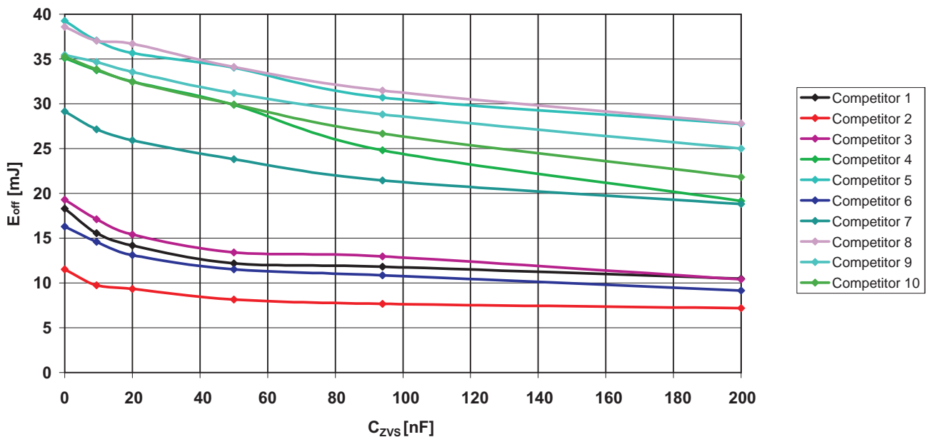
Figure 5.9.13 Comparison of turn-off losses and power loss reduction of the IGBT technology available on the market today (1200 V / 300 A modules); operating point V_{DC} = 600 V, I_C = 300 A under comparable driver conditions
