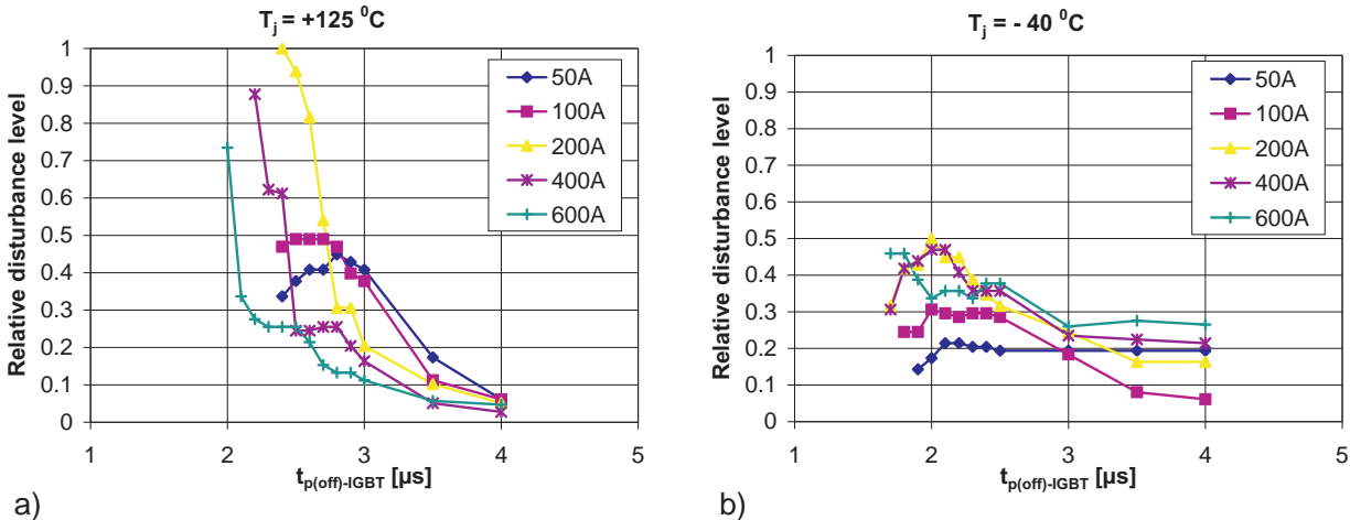
Figure 2.3.14 Relative interference level related to the maximum value at 200 A and 125^\circ C for IGBT turn-off signals of different durations as a function of current and temperature (a) T_j=125^\circ C , b) T_j=-40^\circ C )
