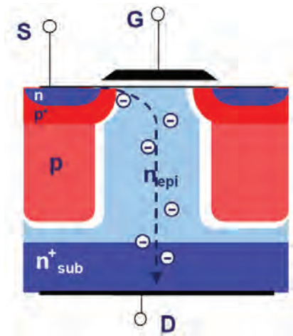
Figure 2.4.21 Layout and functional principle of a superjunction MOSFET (CoolMOS) [25]
