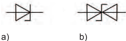
Figure 4.4.12 Circuit symbols for avalanche diode (a) and bipolar suppressor diode (b)
