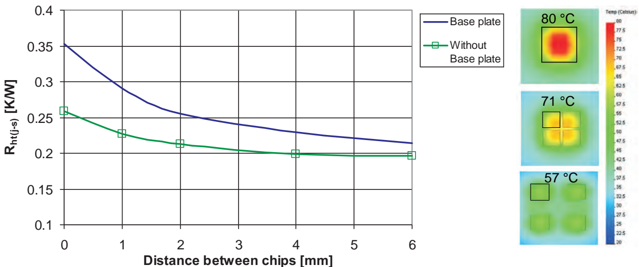
Figure 2.5.21 Thermal resistance R_{\text{ht}(j-s)} of four 36 \text{ mm}^2 chips as a function of the chip distance; (thermal paste thickness: with base plate 100 \mu\text{m} , without 25 \mu\text{m} ), right: simulation of chip temperatures assuming same power loss and chip area but increasing distance (0 mm, 1 mm, 6 mm)
