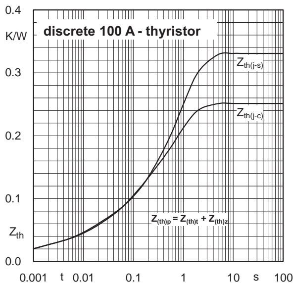
Figure 3.2.4 Z_{th} to case ( Z_{th(j-c)} ) and to heatsink ( Z_{th(j-s)} ) of a discrete 100 A thyristor, and mathematical auxiliary parameter Z_{th(z)} to calculate the temperature fluctuation at line frequency for different current conduction angles and waveforms
