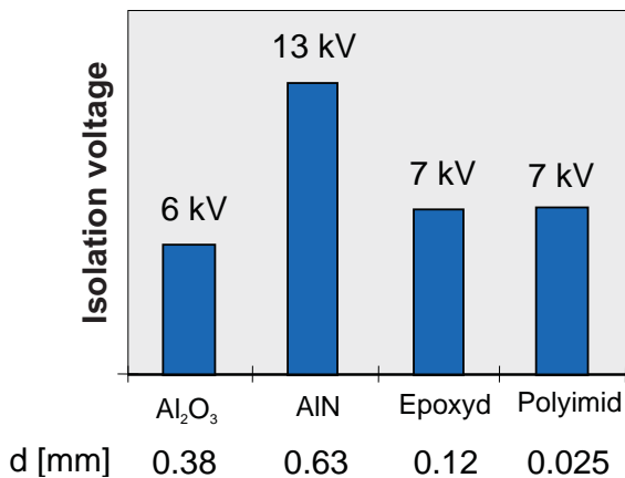
Figure 2.5.12 Insulation voltages for different insulating substrates
