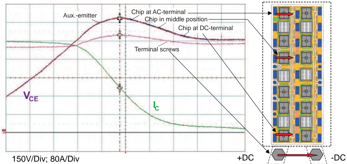
Figure 2.5.26 Overvoltage reading in the SKiM93 during turn-off at different chip positions and the outer terminals at 6.7 kA/μs, time scale = 20 ns/Div
