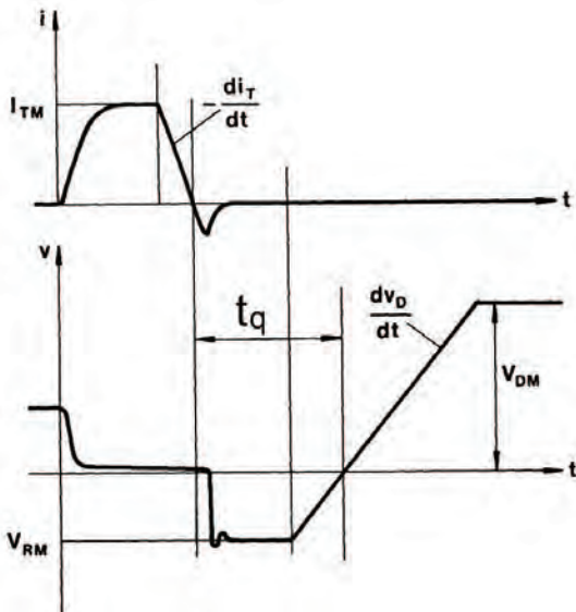
Figure 3.2.23 Main current i and main voltage v of a thyristor over time during commutation from on-state to off-state; the circuit commutated turn-off time t_q is the shortest time interval during which an applied direct off-state voltage will not trigger the thyristor
