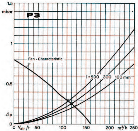
Figure 4.2.10 Diagrams showing pressure drop \Delta p for different lengths l of P3 heat sink as a function of air volume V_{air}/t , as well as the volume of air moved by the fan as a function of the negative pressure (fan characteristic). The points of intersection constitute the resulting volume of air for the given combination of fan / heat sink profile.
