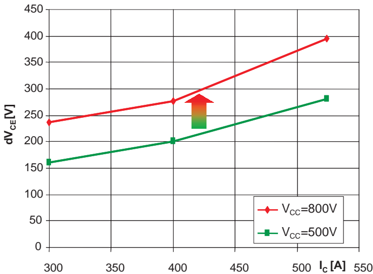
Figure 5.1.3 Impact of the DC link voltage on turn-off overvoltage of a 1200 V / 450 A IGBT module containing "T4" IGBT chips as a function of the collector current for T_c = 25^\circ C
