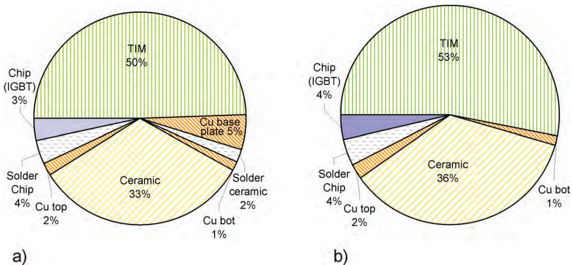
Figure 2.5.16 Influences on the internal thermal resistance of a 1200 V power module, chip surface 9 mm * 9 mm: a) for DBC substrates ( \text{Al}_2\text{O}_3 ) on Cu base plate, 100 \mu\text{m} TIM; b) for DCB substrates ( \text{Al}_2\text{O}_3 ) without Cu base plate, 25 \mu\text{m} TIM
