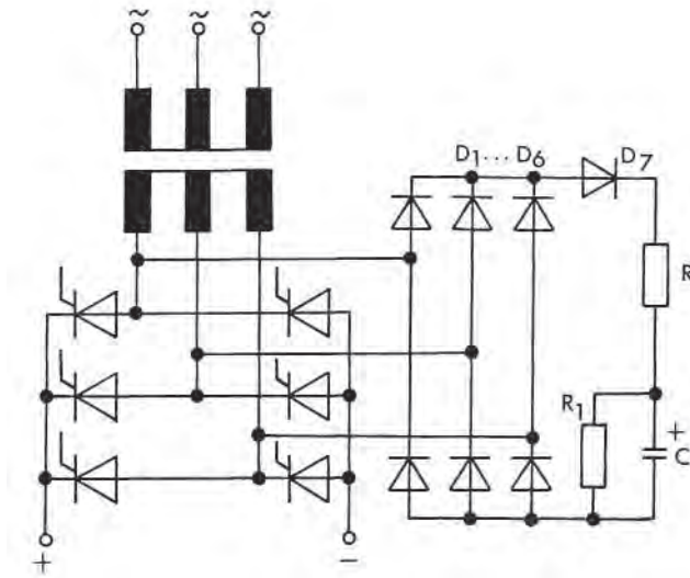
Figure 4.4.9 AC side snubber circuit using auxiliary bridge and auxiliary diode
