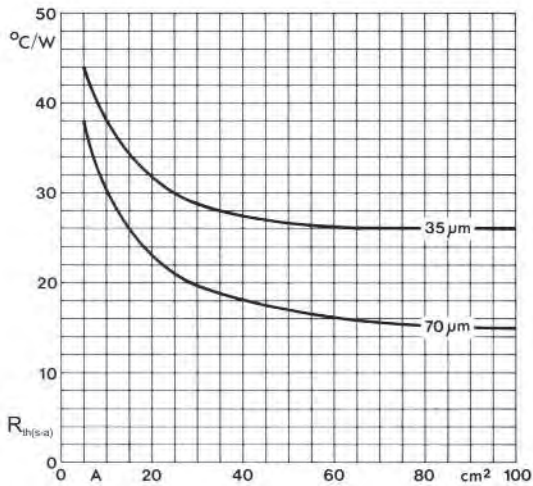
Figure 4.2.3 R_{th(s-a)} of a 1.5 mm thick PCB copper lamination, single-sided lamination, layer thickness 35 \mu\text{m} and 70 \mu\text{m} , as a function of the area A . Any mounting position, provided unobstructed airflow across the entire surface is ensured.
