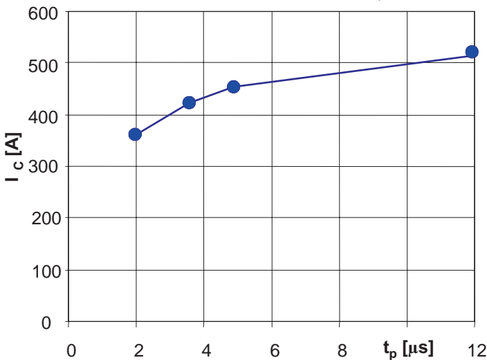
Figure 5.1.4 Necessary current derating to meet V_{CE(max)} for very short turn-on times t_p of a 1200 V-IGBT4 with V_{CC} = 800 V and T_c = 25^\circ C
