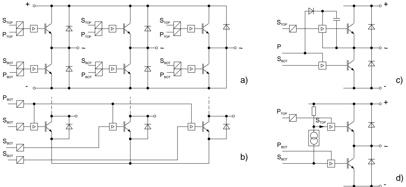
Figure 5.6.12 Selected signal and energy transmission principles STOP, SBOT: control signal for TOP / BOTTOM switch P TOP , P BOT : driving energy for TOP / BOTTOM switch a) Maximum variant, b) Common energy supply for BOTTOM drivers c) Bootstrap principle, d) Level-shifter principle
