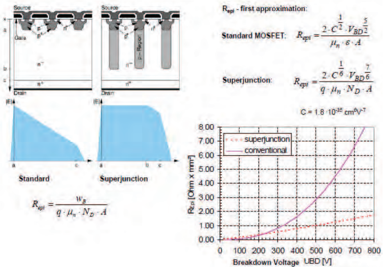
Figure 2.4.22 Comparison of standard and superjunction MOSFET [28]
