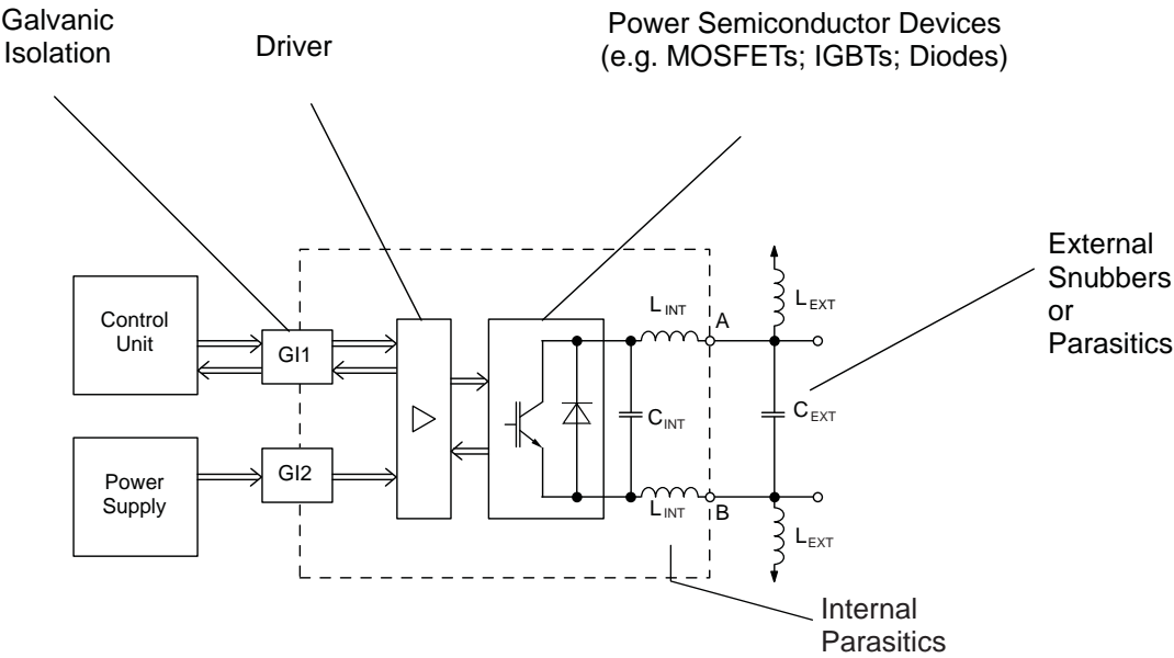
Figure 1.2.1 Power electronic switch system
